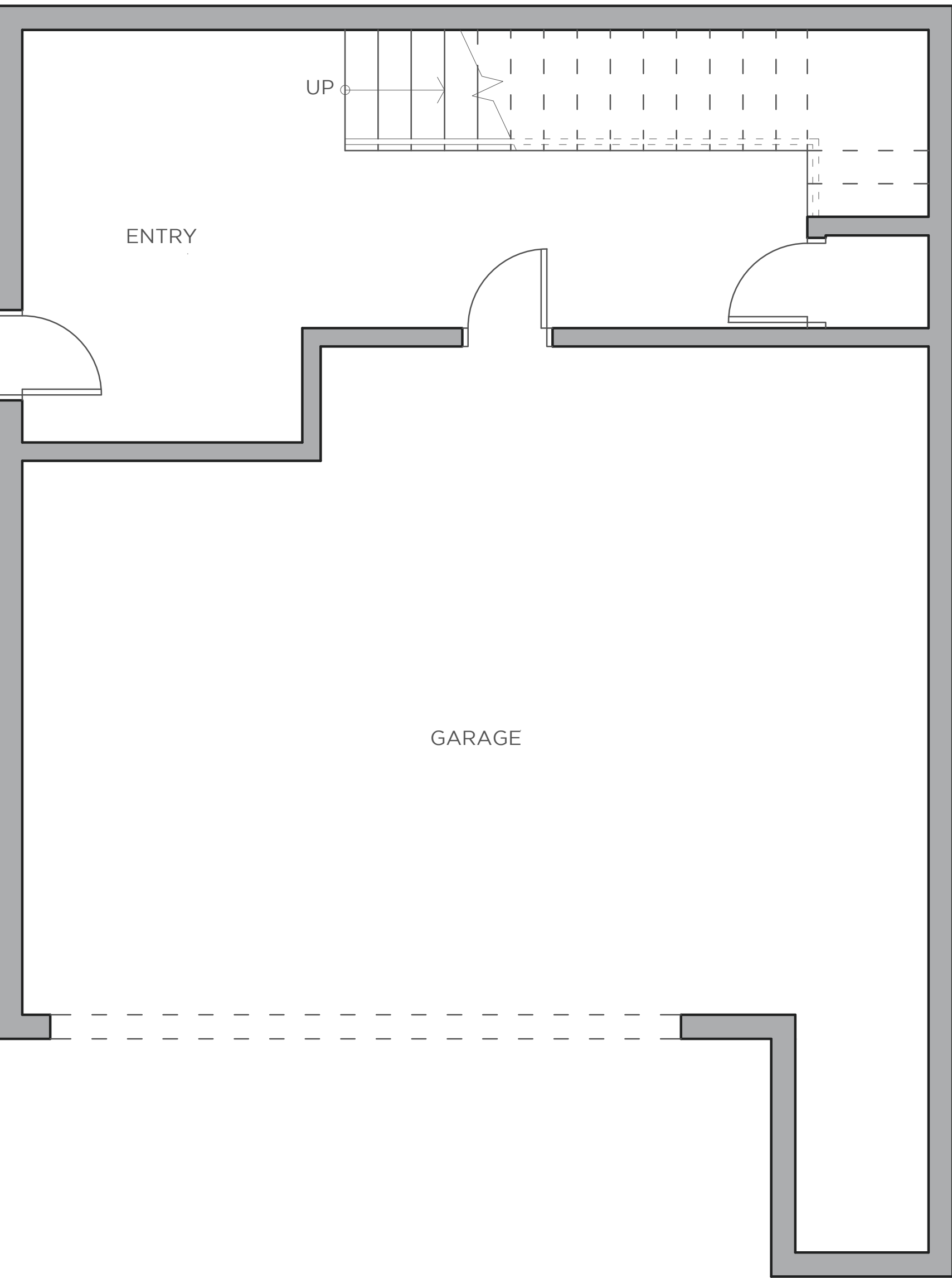
FIRST FLOOR
